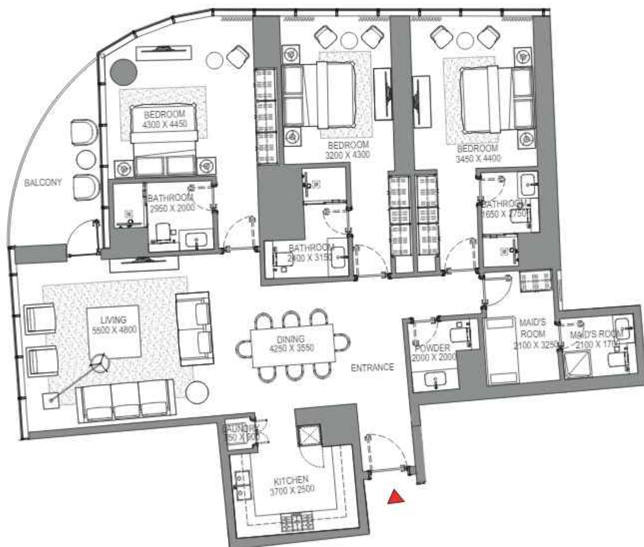
TYPICAL FLOOR PLAN LEVEL II-23
